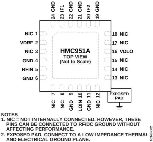
Figure 2. Pin Configuration
