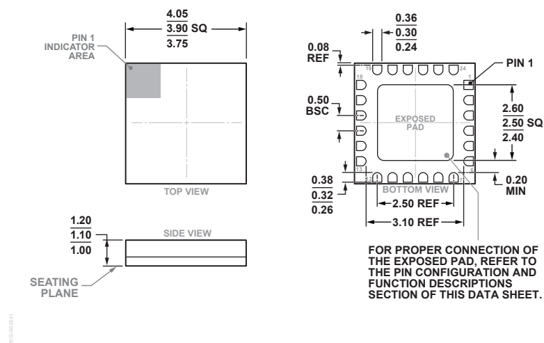
24-Terminal Ceramic Leadless Chip Carrier [LCC] (E-24-2)
