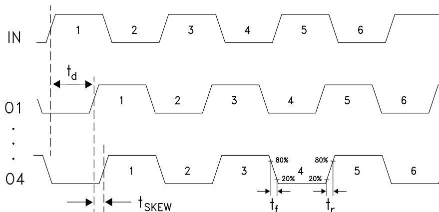
Timing Diagram
