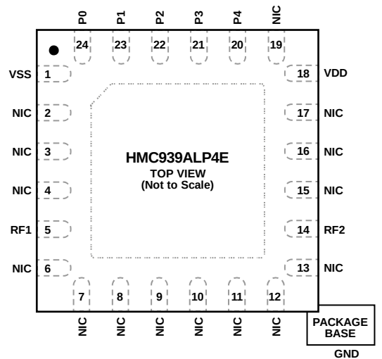
Figure 2. Pin Configuration
