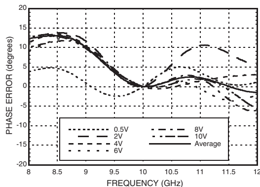
Phase Error vs. Frequency, Fmean = 10 GHz [1]
