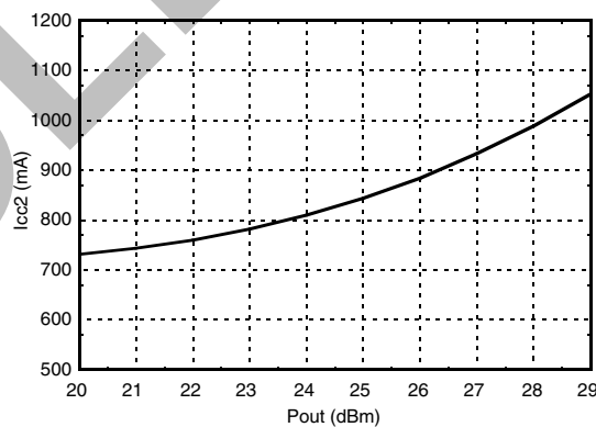
I_{cc2} vs. Output Power @ 700 mA
