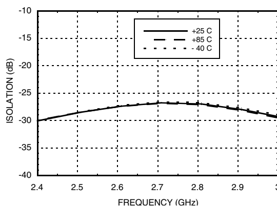
Reverse Isolation vs. Temperature 700 mA
