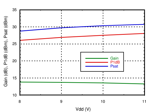
Gain & Power vs. Vdd @ 18 GHz
