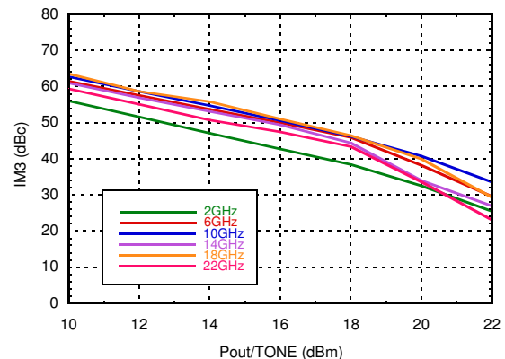
Output IM3 @ Vdd = +10 V
