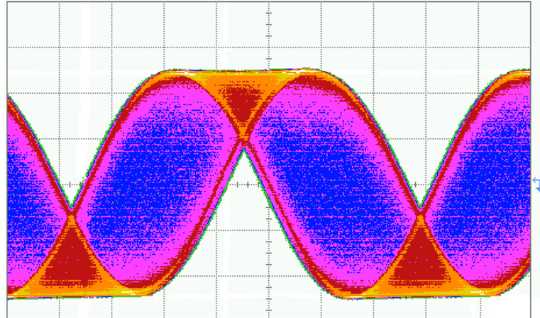
Output Eye Diagram Continuous Snapshot for 15 GHz Input Signal
