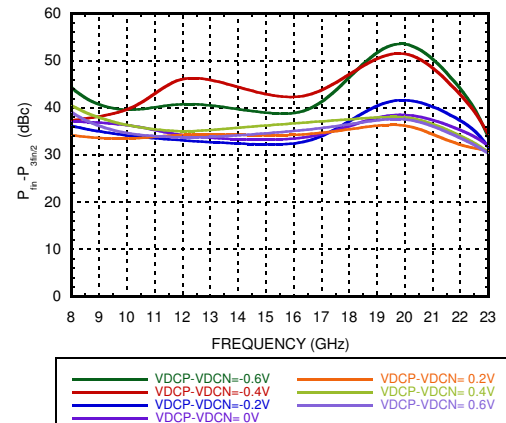
P_{fin} - P_{3fin/2} Output Power Difference vs. Control Voltage [1][2][5]
