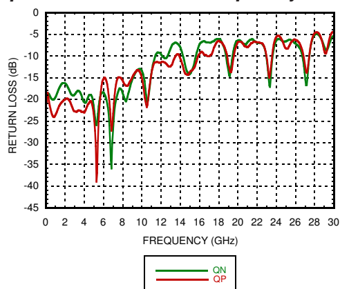
Output Return Loss vs. Frequency [1][4]
