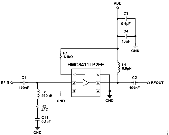
Figure 71. Typical Application Circuit
