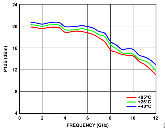
Figure 34. P1dB vs. Frequency, 1 GHz to 12 GHz, for Various Temperatures, V_{DD} = 5\text{ V} , I_{DQ} = 55\text{ mA}
