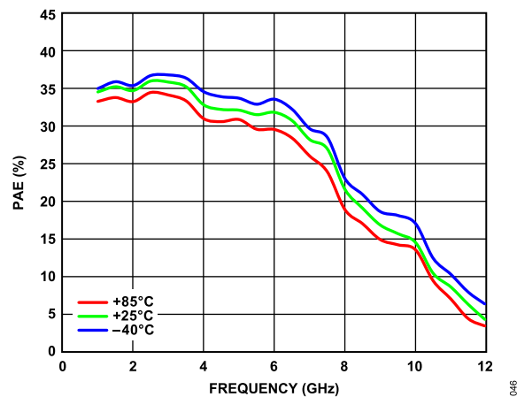
Figure 46. PAE vs. Frequency, 1 GHz to 12 GHz, for Various Temperatures, V_{DD} = 5\text{ V} , I_{DQ} = 55\text{ mA}
