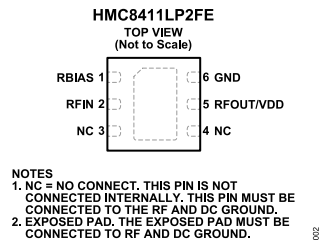
Figure 2. Pin Configuration
