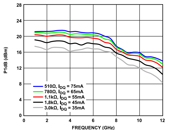
Figure 36. P1dB vs. Frequency, 1 GHz to 12 GHz, for Various Bias Resistor Values and I_{DQ} , V_{DD} = 5\text{ V}
