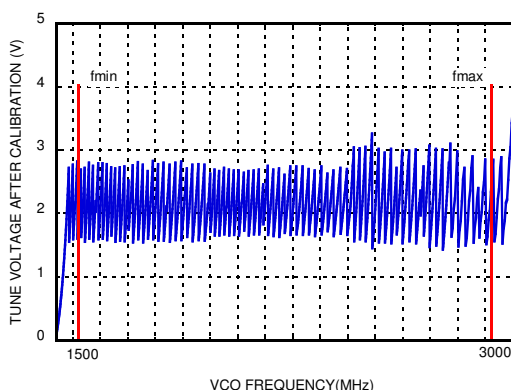
Figure 6. Typical Tuning Voltage After Calibration at F o
