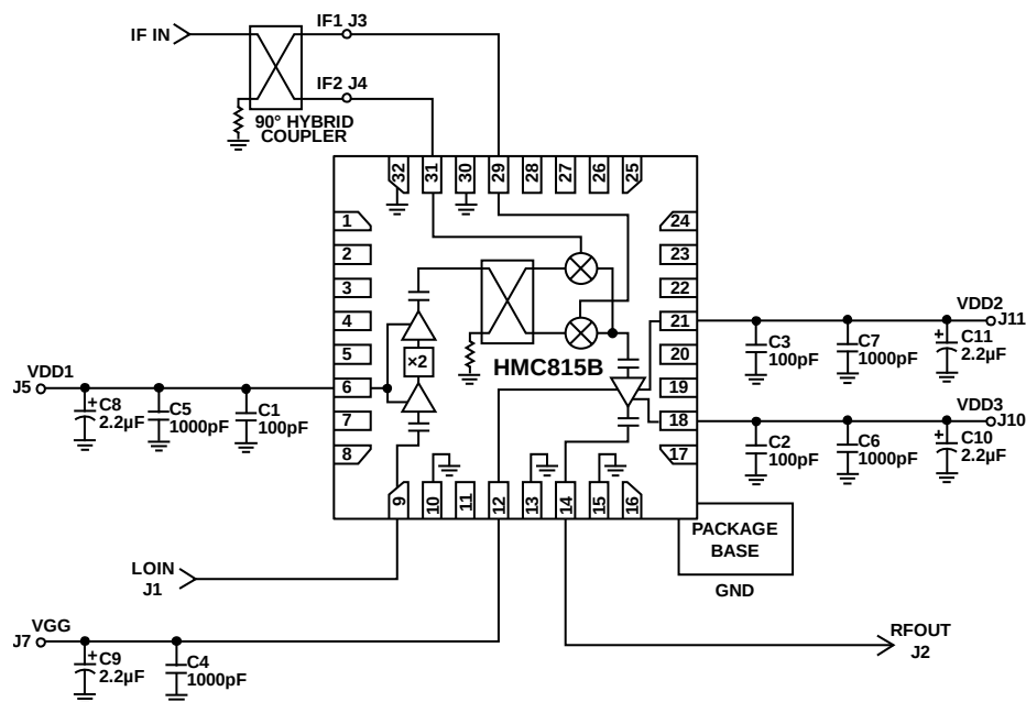
Figure 104. Typical Application Circuit
