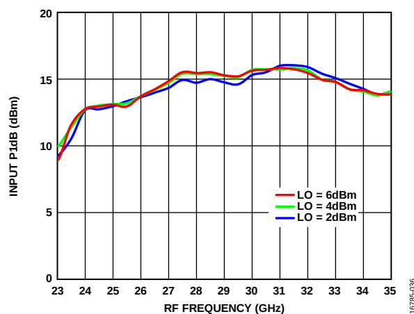
Figure 38. Input P1dB vs. RF Frequency at Various LO Power Levels, T_A = 25^\circ\text{C}
