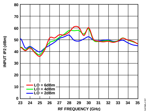
Figure 37. Input IP2 vs. RF Frequency at Various LO Power Levels, T_A = 25^\circ\text{C}
