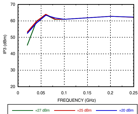
Input IP3 vs. Tone Power @ Vdd = +5V
