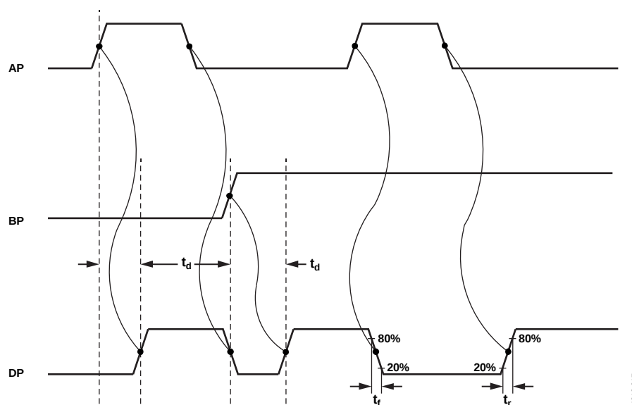
Figure 17. Timing Diagram
