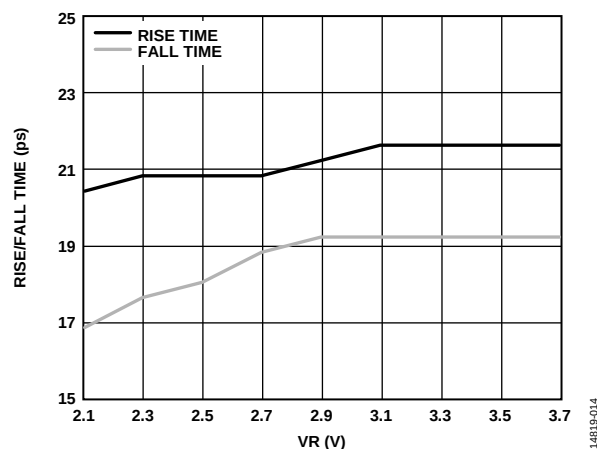
Figure 13. Rise/Fall Time vs. VR, Frequency = 13 GHz
