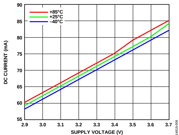
Figure 8. DC Current vs. Supply Voltage, VR = 3.3 V, Frequency = 13 GHz
