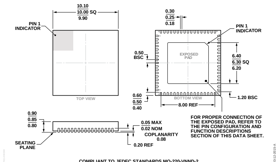
Figure 54. 68-Lead Lead Frame Chip Scale Package [LFCSP_VQ] 10 mm x 10 mm Body, Very Thin Quad (HCP-68-1) Dimensions shown in millimeters
