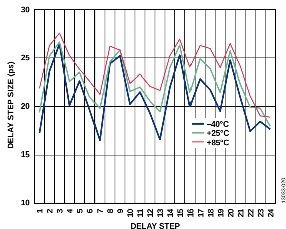
Figure 18. Analog Delay Step Size vs. Delay Step over Temperature, LVPECL at 1474.56 MHz
