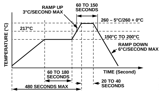
Figure 51. Pb-Free Reflow Solder Profile
