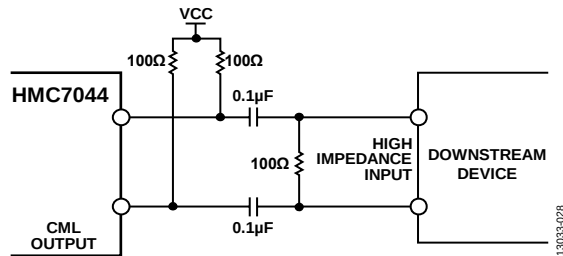
Figure 28. AC-Coupled CML (Configured High-Z) Output Driver
