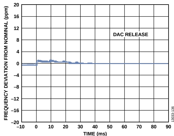
Figure 40. DAC Assisted Release
