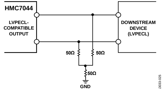
Figure 32. DC-Coupled LVPECL Output Driver
