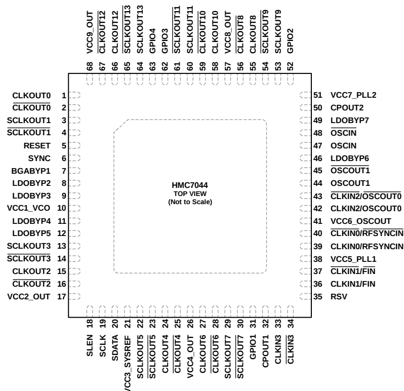
Figure 2. Pin Configuration
