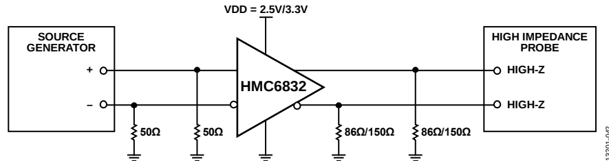
Figure 39. Test Circuit for DC LVPECL Measurements, 86 Ω Termination Used for VDD = 2.5 V; 150 Ω Termination Used for VDD = 3.3 V
