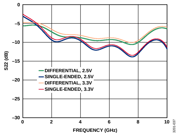
Figure 34. LVPECL S Parameters ( S_{22} ), Network Analyzer Gating Used to Remove Input and Output Impedance Mismatch and Board Loss
