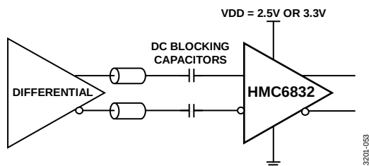
Figure 50. Differential Input AC-Coupled Interface
