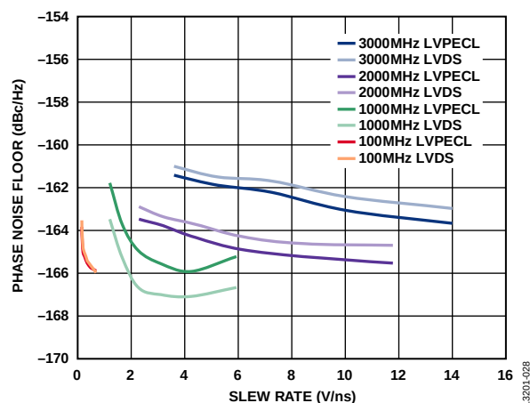
Figure 25. Phase Noise Floor vs. Slew Rate for Carrier Frequencies and Output Configurations, LVPECL R_{TERM} = 150 \Omega ; LVDS R_{TERM} = 100 \Omega
