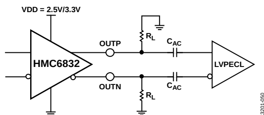
Figure 47. Recommended Interface Diagram
