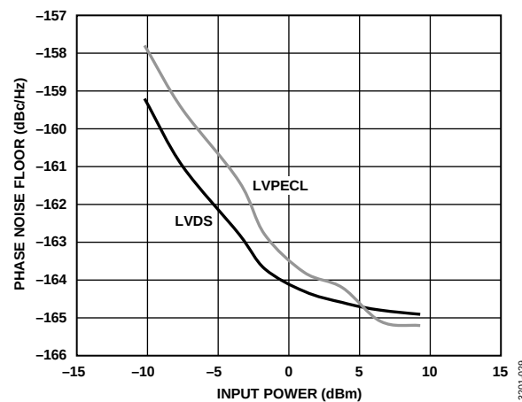
Figure 26. Phase Noise Floor at 1.6 GHz vs. Input Power, LVPECL R_{TERM} = 150 \Omega ; LVDS R_{TERM} = 100 \Omega
