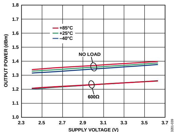
Figure 36. VAC_REF Output Power vs. Supply Voltage for Various Temperatures and Current Loads; 600 \Omega Signifies 2 mA Output Load
