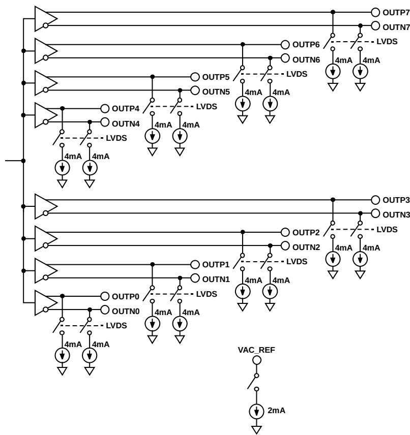
Figure 46. Output Stage Block Diagram
