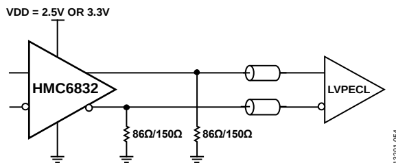
Figure 51. LVPECL Output DC Termination Interface (86 Ω Termination Can Be Used at 2.5 V Only)
