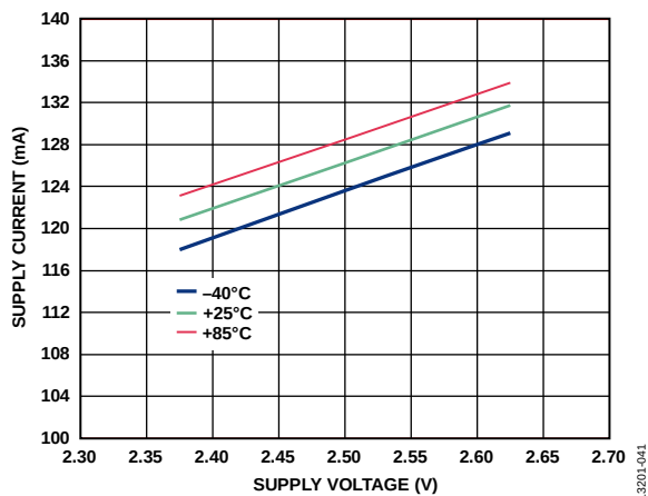
Figure 38. LVDS Supply Current vs. Supply Voltage for Various Temperatures
