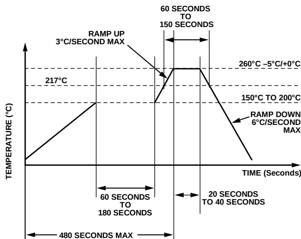
Figure 53. LFCSP Pb-Free Reflow Profile
