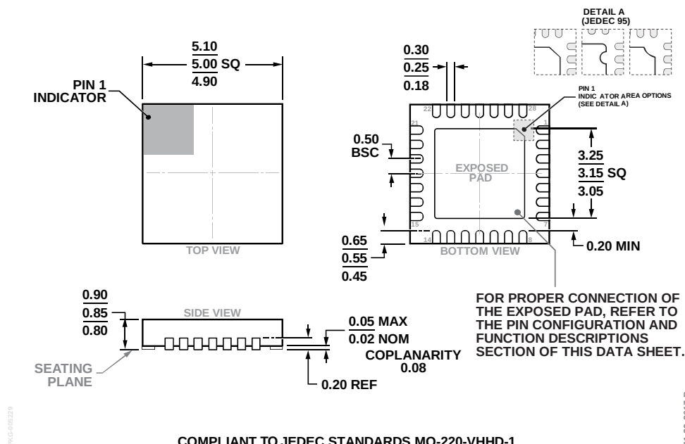
Figure 56. 28-Lead Lead Frame Chip Scale Package [LFCSP] 5 mm × 5 mm Body and 0.85 mm Package Height (HCP-28-1)
