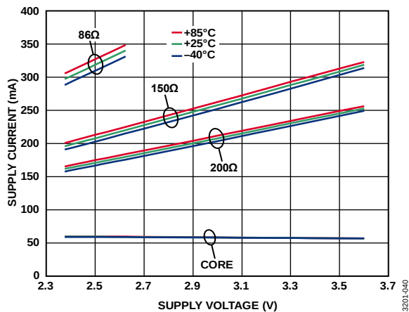
Figure 37. LVPECL Supply Current vs. Supply Voltage for Various Temperatures and R_{TERM} Values
