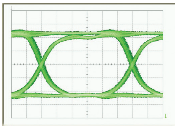
Eye Diagram
