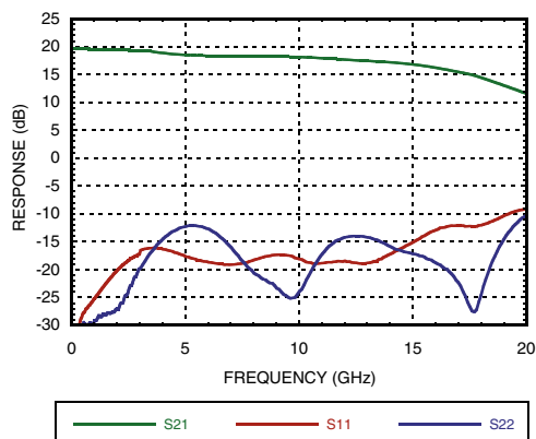
Gain &amp; Return Loss
