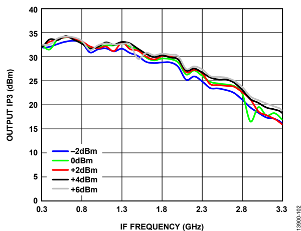
Figure 102. Output IP3 vs. IF Frequency over LO Powers, LO Frequency = 7 GHz, T_A = 25^\circ\text{C} , Voltage Control = -4 V
