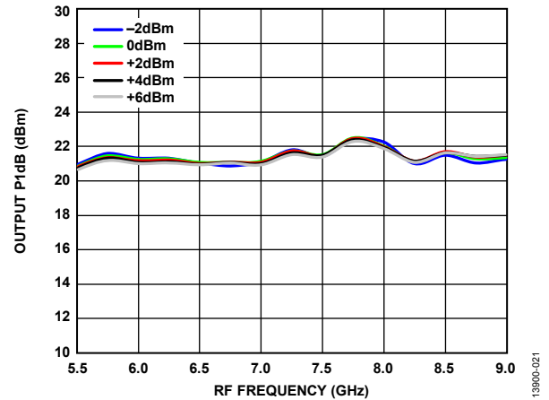
Figure 21. Output P1dB vs. RF Frequency over LO Powers, T_A = 25^\circ\text{C} , Voltage Control = -4 V
