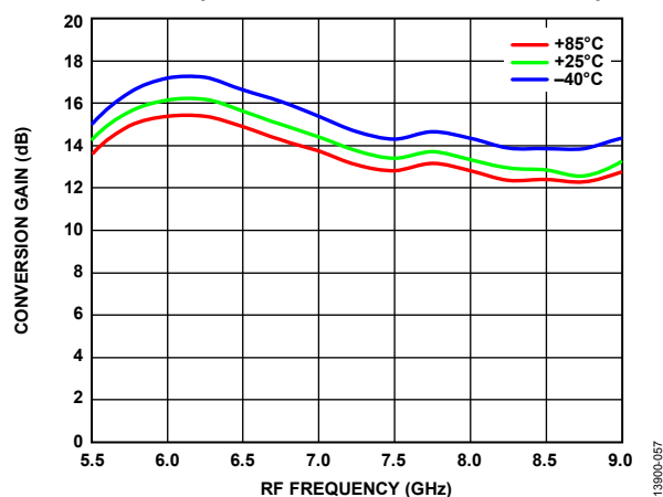
Figure 57. Conversion Gain vs. RF Frequency over Temperatures, LO Power = 4 dBm, Voltage Control = -4 V
