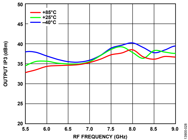
Figure 28. Output IP3 vs. RF Frequency over Temperatures, LO Power = 4 dBm, Voltage Control = -4 V
