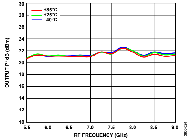
Figure 20. Output P1dB vs. RF Frequency over Temperatures, LO Power = 4 dBm, Voltage Control = -4 V
