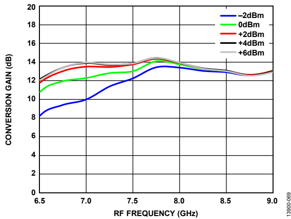
Figure 69. Conversion Gain vs. RF Frequency over LO Powers, T_A = 25^\circ\text{C} , Voltage Control = -4 V
