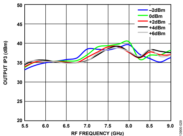
Figure 29. Output IP3 vs. RF Frequency over LO Powers T_A = 25^\circ\text{C} , Voltage Control = -4 V
