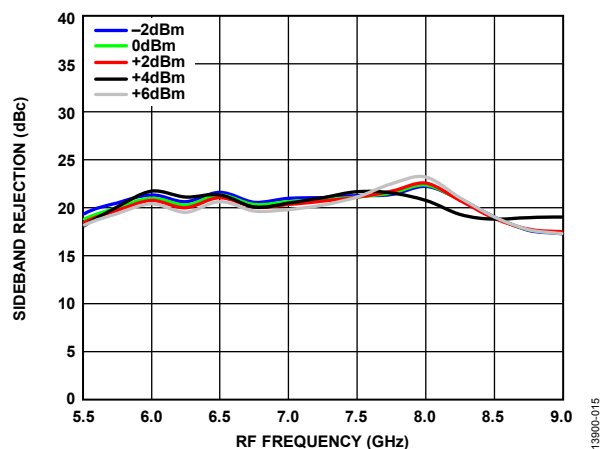
Figure 15. Sideband Rejection vs. RF Frequency over LO Powers, T_A = 25^\circ\text{C} , Voltage Control = -4 V
