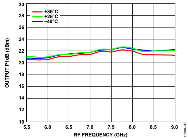
Figure 42. Output P1dB vs. RF Frequency over Temperatures, LO Power = 4 dBm, Voltage Control = -4 V
