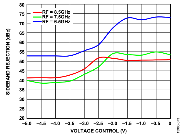
Figure 73. Sideband Rejection vs. Voltage Control over RF, T_A = 25^\circ\text{C} , LO Power = 4 dBm
