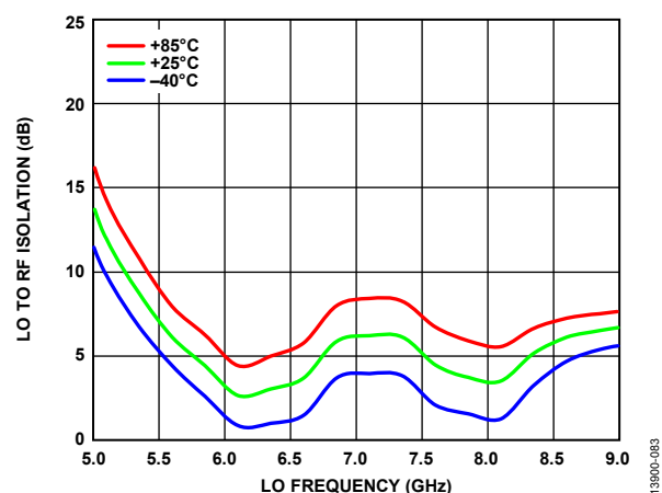
Figure 81. LO to RF Isolation vs. LO Frequency over Temperatures, LO Power = 4 dBm, Voltage Control = -4 V
