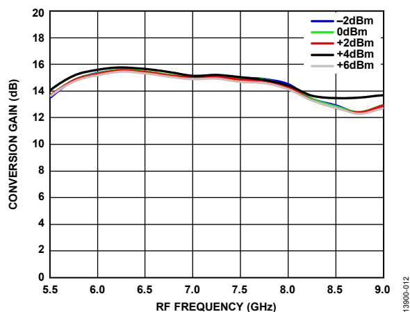
Figure 12. Conversion Gain vs. RF Frequency over LO Powers, T_A = 25^\circ\text{C} , Voltage Control = -4 V
