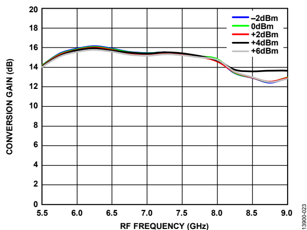
Figure 23. Conversion Gain vs. RF Frequency over LO Powers, T_A = 25^\circ\text{C} , Voltage Control = -4 V
