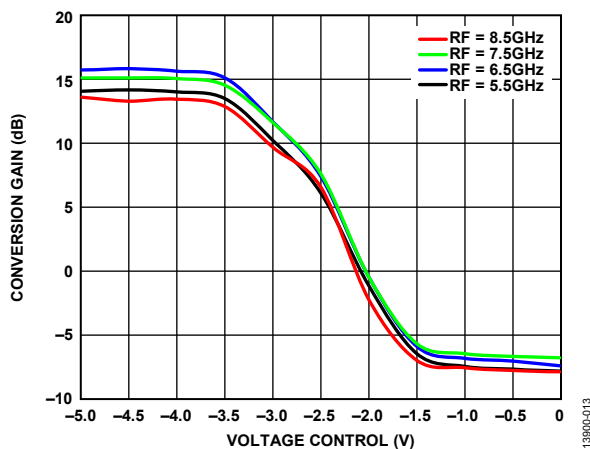
Figure 13. Conversion Gain vs. Voltage Control over RF, T_A = 25^\circ\text{C} , LO Power = 4 dBm
