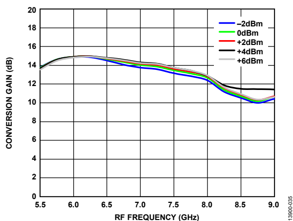
Figure 34. Conversion Gain vs. RF Frequency over LO Powers, T_A = 25^\circ\text{C} , Voltage Control = -4 V
