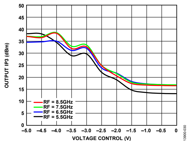
Figure 30. Output IP3 vs. Voltage Control over RF, T_A = 25^\circ\text{C} , LO Power = 4 dBm
