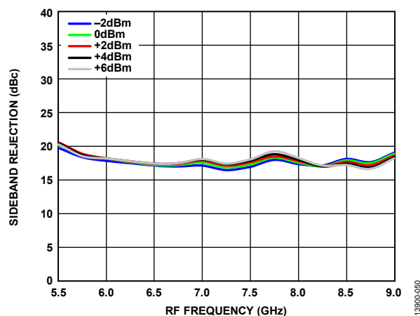
Figure 50. Sideband Rejection vs. RF Frequency over LO Powers, T_A = 25^\circ\text{C} , Voltage Control = -4 V
