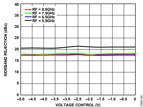
Figure 51. Sideband Rejection vs. Voltage Control over RF, T_A = 25^\circ\text{C} , LO Power = 4 dBm
