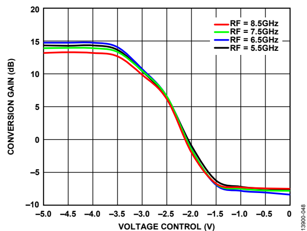
Figure 48. Conversion Gain vs. Voltage Control over RF, T_A = 25^\circ\text{C} , LO Power = 4 dBm
