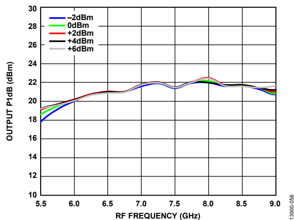
Figure 56. Output P1dB vs. RF Frequency over LO Powers, T_A = 25^\circ\text{C} , Voltage Control = -4 V
