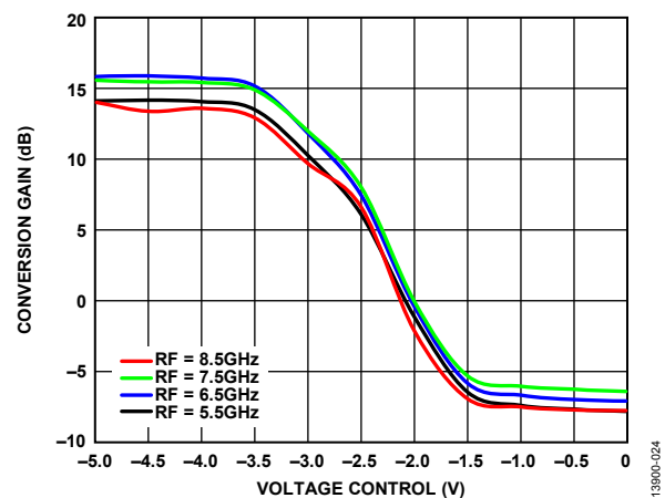
Figure 24. Conversion Gain vs. Voltage Control over RF, T_A = 25^\circ\text{C} , LO Power = 4 dBm
