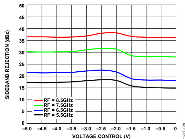
Figure 38. Sideband Rejection vs. Voltage Control over RF, T_A = 25^\circ\text{C} , LO Power = 4 dBm
