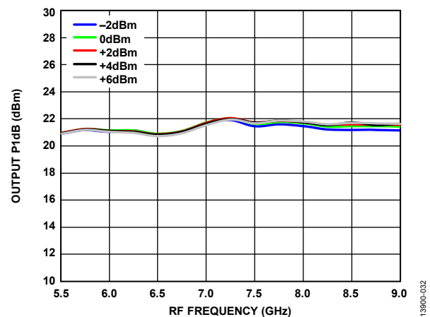
Figure 32. Output P1dB vs. RF Frequency over LO Powers, T_A = 25^\circ\text{C} , Voltage Control = -4 V
