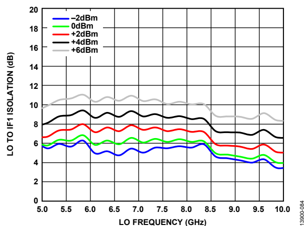
Figure 82. LO to IF1 Isolation vs. LO Frequency over LO Powers, T_A = 25^\circ\text{C} , Voltage Control = -4 V
