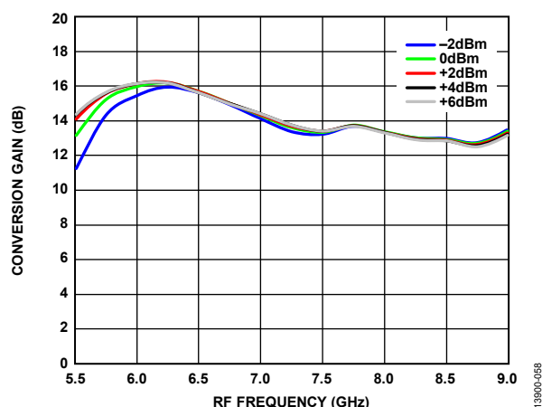
Figure 58. Conversion Gain vs. RF Frequency over LO Powers, T_A = 25^\circ\text{C} , Voltage Control = -4 V
