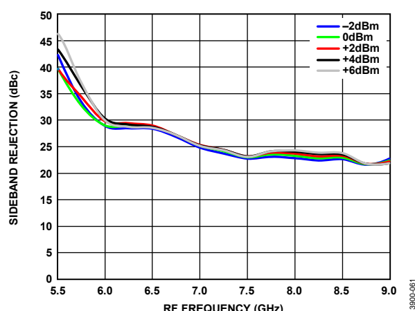
Figure 61. Sideband Rejection vs. RF Frequency over LO Powers, T_A = 25^\circ\text{C} , Voltage Control = -4 V
