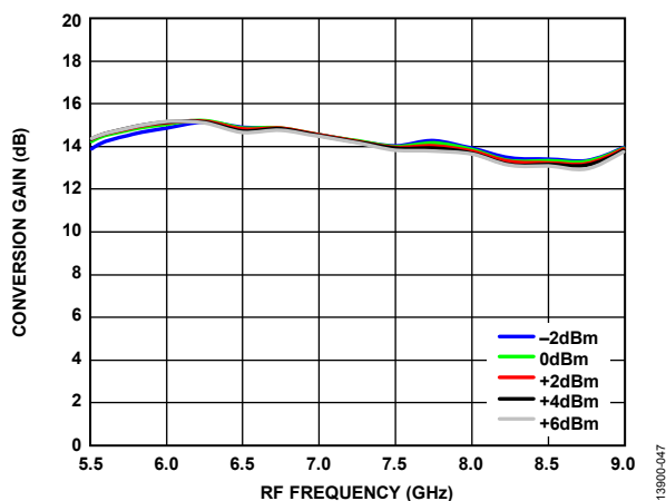
Figure 47. Conversion Gain vs. RF Frequency over LO Powers, T_A = 25^\circ\text{C} , Voltage Control = -4 V
