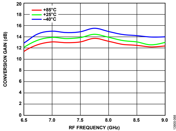
Figure 68. Conversion Gain vs. RF Frequency over Temperatures, LO Power = 4 dBm, Voltage Control = -4 V
