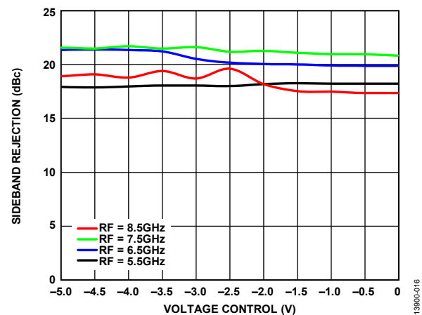
Figure 16. Sideband Rejection vs. Voltage Control over RF, T_A = 25^\circ\text{C} , LO Power = 4 dBm
