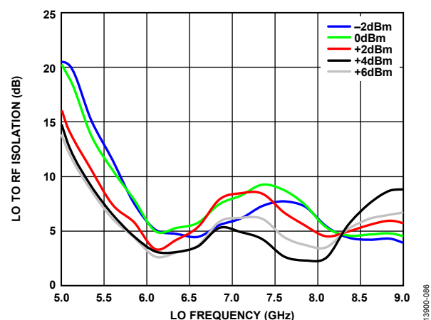
Figure 84. LO to RF Isolation vs. LO Frequency over LO Powers, T_A = 25^\circ\text{C} , Voltage Control = -4 V
