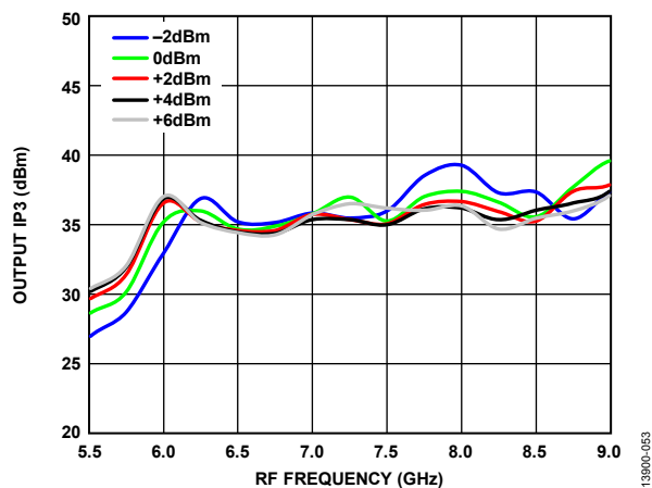
Figure 53. Output IP3 vs. RF Frequency over LO Powers T_A = 25^\circ\text{C} , Voltage Control = -4 V
