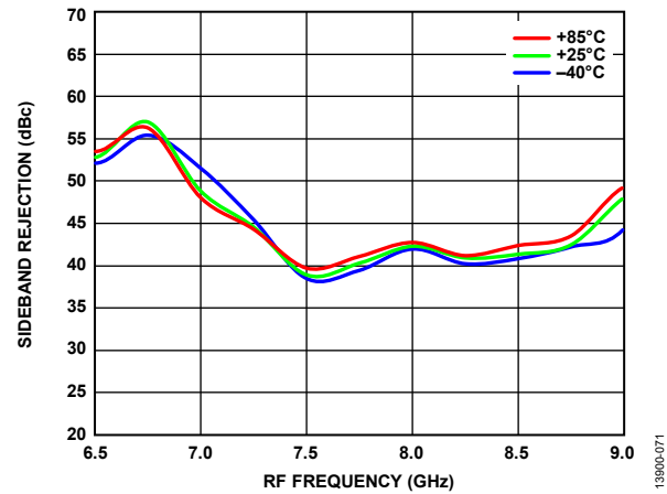
Figure 71. Sideband Rejection vs. RF Frequency over Temperatures, Voltage Control = -4 V
