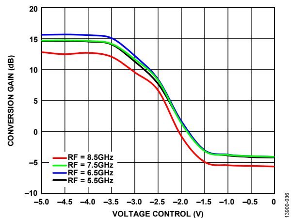
Figure 35. Conversion Gain vs. Voltage Control over RF, T_A = 25^\circ\text{C} , LO Power = 4 dBm
