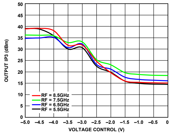
Figure 19. Output IP3 vs. Voltage Control over RF Frequencies, T_A = 25^\circ\text{C} , LO Power = 4 dBm
