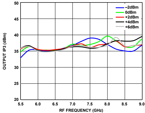
Figure 18. Output IP3 vs. RF Frequency over LO Powers, T_A = 25^\circ\text{C} , Voltage Control = -4 V
