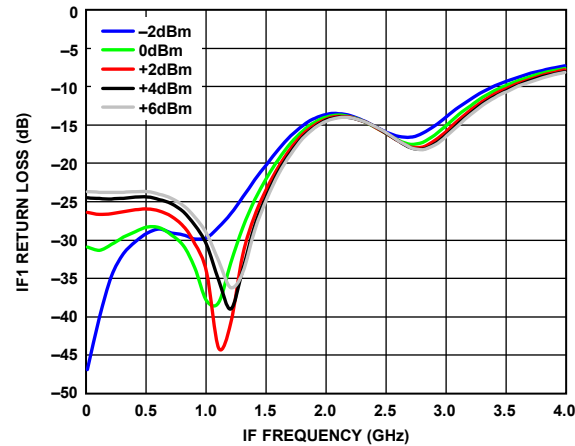
Figure 95. IF1 Return Loss vs. IF Frequency over LO Powers, LO Frequency = 7 GHz, T_A = 25^\circ\text{C} , Voltage Control = -4 V
