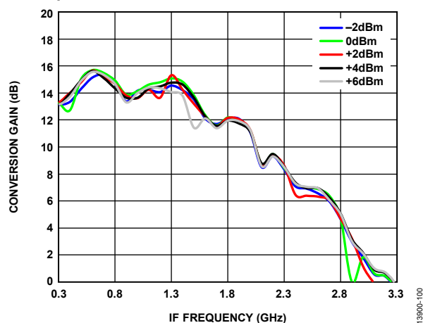
Figure 100. Conversion Gain vs. IF Frequency over LO Powers, LO Frequency = 7 GHz, T_A = 25^\circ\text{C} , Voltage Control = -4 V
