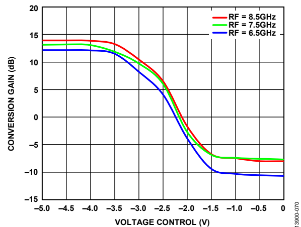
Figure 70. Conversion Gain vs. Voltage Control over RF, T_A = 25^\circ\text{C} , LO Power = 4 dBm
