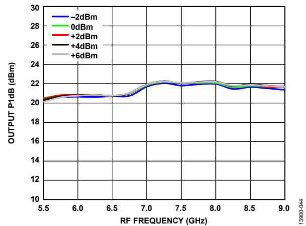
Figure 43. Output P1dB vs. RF Frequency over LO Powers, T_A = 25^\circ\text{C} , Voltage Control = -4 V
