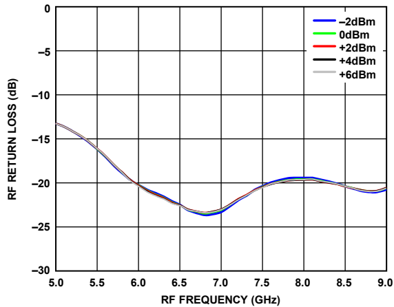
Figure 92. RF Return Loss vs. RF Frequency over LO Powers, LO Frequency = 7 GHz, T_A = 25^\circ\text{C} , Voltage Control = -4 V
