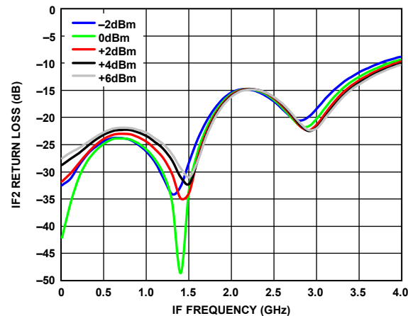
Figure 96. IF2 Return Loss vs. IF Frequency over LO Powers, LO Frequency = 7 GHz, T_A = 25^\circ\text{C} , Voltage Control = -4 V
