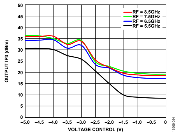
Figure 54. Output IP3 vs. Voltage Control over RF, T_A = 25^\circ\text{C} , LO Power = 4 dBm
