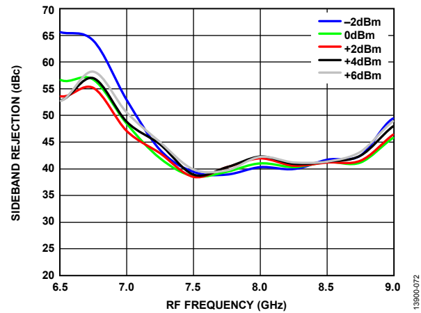
Figure 72. Sideband Rejection vs. RF Frequency over LO Powers, T_A = 25^\circ\text{C} , Voltage Control = -4 V
