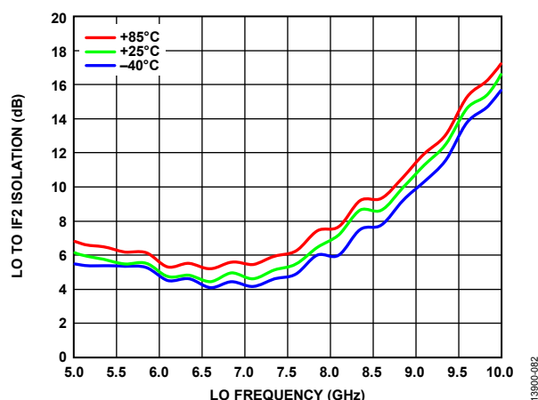
Figure 80. LO to IF2 Isolation vs. LO Frequency over Temperatures, IF = 350 MHz, LO Power = 4 dBm, Voltage Control = -4 V
