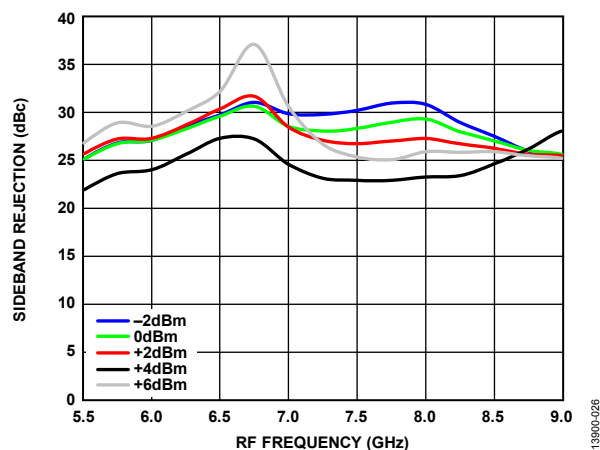
Figure 26. Sideband Rejection vs. RF Frequency over LO Powers, T_A = 25^\circ\text{C} , Voltage Control = -4 V
