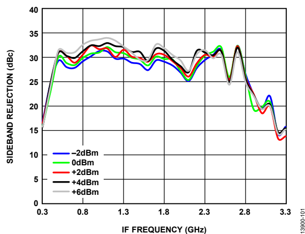
Figure 101. Sideband Rejection vs. IF Frequency over LO Powers, LO Frequency = 7 GHz, T_A = 25^\circ\text{C} , Voltage Control = -4 V
