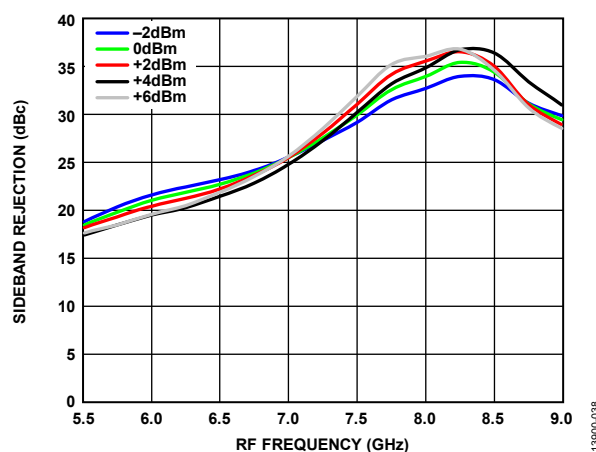
Figure 37. Sideband Rejection vs. RF Frequency over LO Powers, T_A = 25^\circ\text{C} , Voltage Control = -4 V
