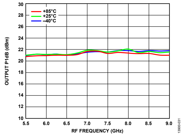
Figure 31. Output P1dB vs. RF Frequency over Temperatures, LO Power = 4 dBm, Voltage Control = -4 V
