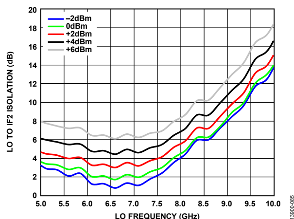
Figure 83. LO to IF2 Isolation vs. LO Frequency over LO Powers, T_A = 25^\circ\text{C} , Voltage Control = -4 V
