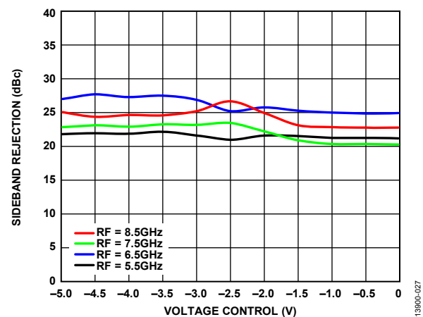
Figure 27. Sideband Rejection vs. Voltage Control over RF, T_A = 25^\circ\text{C} , LO Power = 4 dBm
