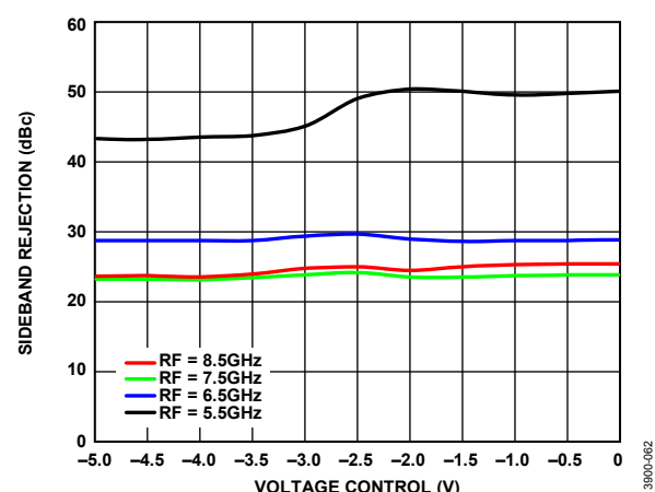
Figure 62. Sideband Rejection vs. Voltage Control over RF, T_A = 25^\circ\text{C} , LO Power = 4 dBm
