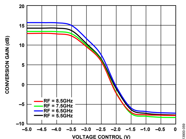
Figure 59. Conversion Gain vs. Voltage Control over RF, T_A = 25^\circ\text{C} , LO Power = 4 dBm
