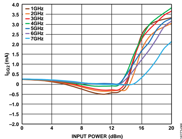
Figure 66. Gate 2 Current ( I_{GG2} ) vs. Input Power for Various Frequencies, V_{DD} = 12\text{ V} , V_{GG2} = 5\text{ V} , V_{GG1} = \text{GND}
