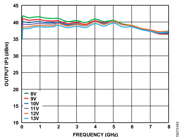
Figure 43. Output IP3 vs. Frequency for Various Supply Voltages ( V_{DD} ), V_{GG2} = Open , V_{GG1} = GND , P_{OUT}/Tone = 10 dBm
