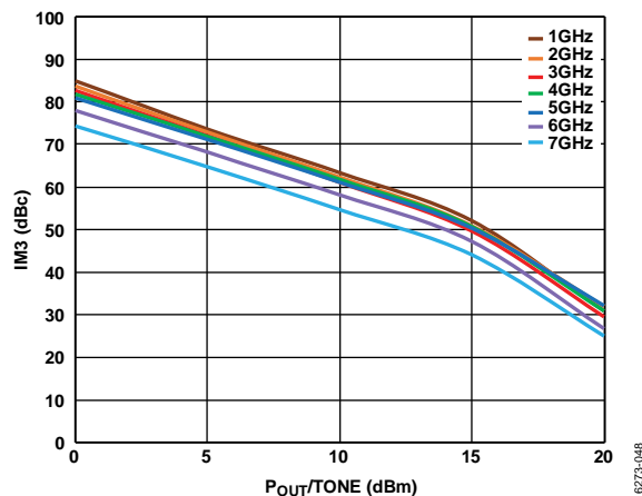
Figure 48. IM3 vs. P_{OUT}/Tone , V_{DD} = 8\text{ V} , V_{GG2} = \text{Open} , V_{GG1} = \text{GND}
