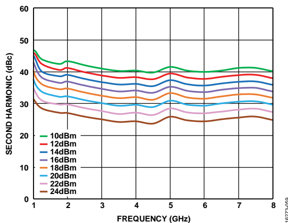
Figure 59. Second Harmonic vs. Frequency for Various P_{OUT} Values, V_{DD} = 12 V, V_{GG2} = \text{Open} , V_{GG1} = \text{GND} (Self Biased)
