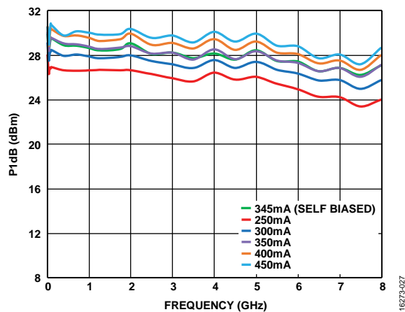
Figure 27. P1dB vs. Frequency for Various Supply Currents ( I_{DD} ), Externally Biased Mode, V_{DD} = 12 V, V_{GG2} = \text{Open} , Controlled V_{GG1}
