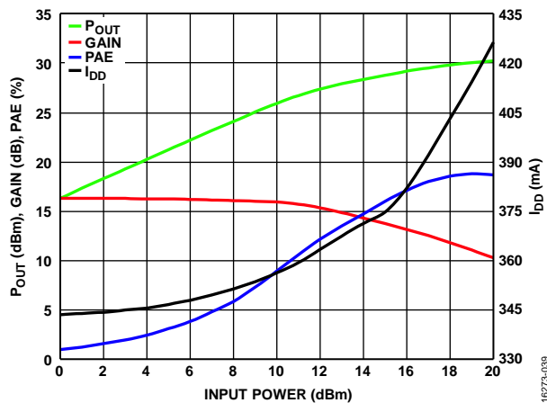
Figure 39. P_{OUT} , Gain, PAE, and I_{DD} vs. Input Power, 6 GHz, V_{DD} = 12 V, V_{GG1} = GND , V_{GG2} = Open
