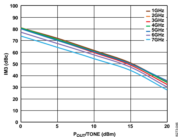
Figure 46. Third-Order Intermodulation Distortion Relative to Carrier (IM3) vs. P_{OUT}/Tone , V_{DD} = 9\text{ V} , V_{GG2} = \text{Open} , V_{GG1} = \text{GND}
