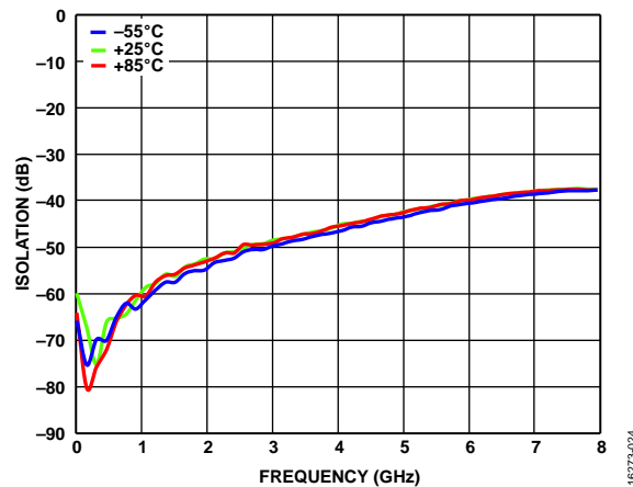
Figure 24. Reverse Isolation vs. Frequency for Various Temperatures, Self Biased Mode, V_{DD} = 12\text{ V} , V_{GG2} = \text{Open} , V_{GG1} = \text{GND}
