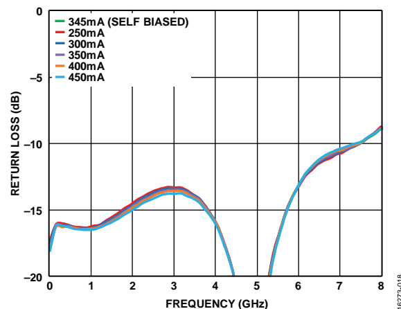
Figure 18. Input Return Loss vs. Frequency for Various Supply Currents ( I_{DD} ), Externally Biased Mode, V_{DD} = 12 V, V_{GG2} = Open, Controlled V_{GG1}
