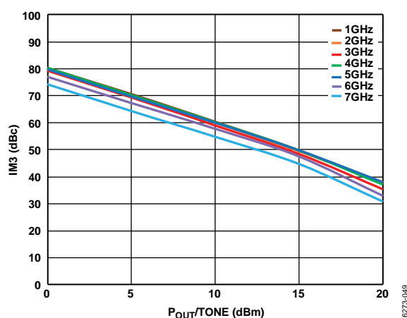
Figure 49. IM3 vs. P_{OUT}/Tone , V_{DD} = 10\text{ V} , V_{GG2} = \text{Open} , V_{GG1} = \text{GND}
