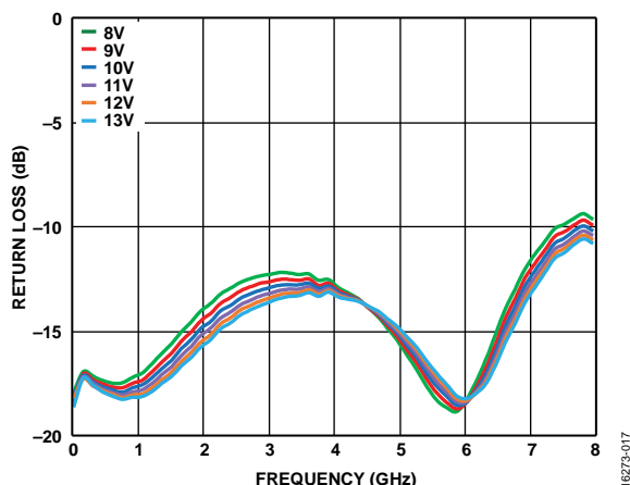
Figure 17. Output Return Loss vs. Frequency for Various Supply Voltages ( V_{DD} ), Self Biased Mode, V_{GG2} = Open, V_{GG1} = GND
