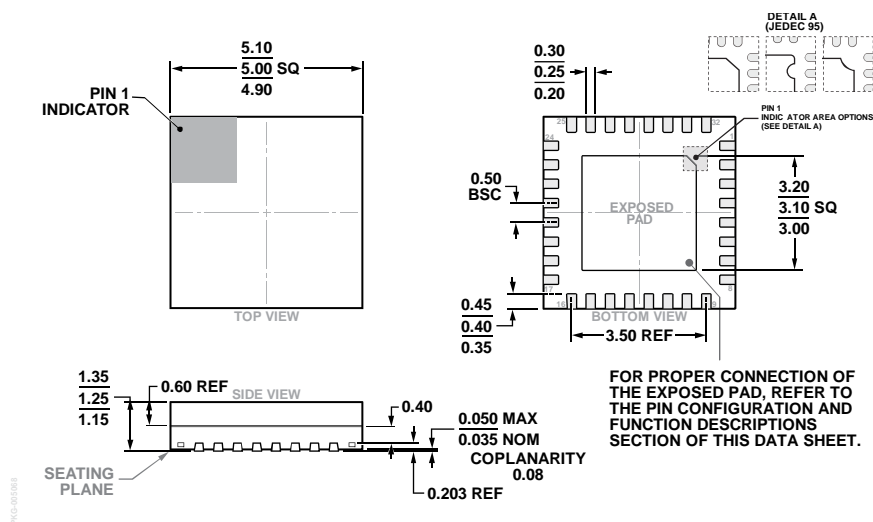
Figure 72. 32-Lead Lead Frame Chip Scale Package, Premolded Cavity [LFCSP_CAV] 5 mm × 5 mm Body and 1.25 mm Package Height (CG-32-2)
