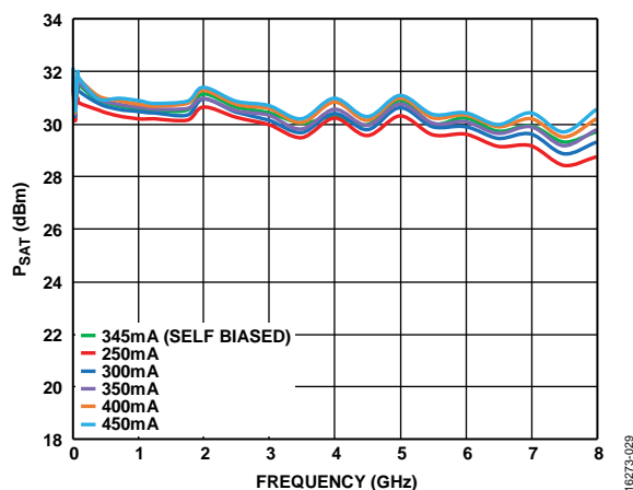
Figure 29. P_{SAT} vs. Frequency for Various Supply Currents ( I_{DD} ), V_{DD} = 12 V, V_{GG2} = \text{Open} , Controlled V_{GG1}
