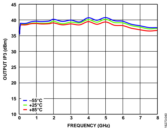
Figure 40. Output IP3 vs. Frequency for Various Temperatures, P_{OUT}/Tone = 10 dBm, Self Biased Mode, V_{DD} = 12 V, V_{GG2} = Open , V_{GG1} = GND
