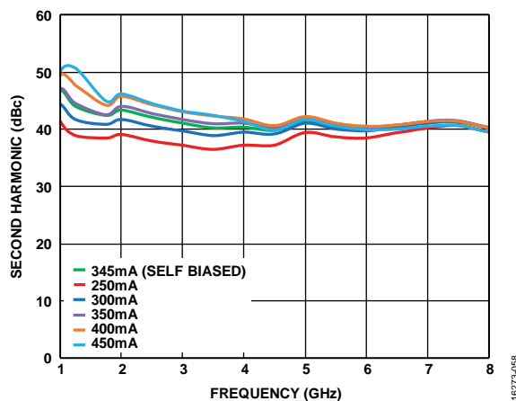
Figure 58. Second Harmonic vs. Frequency for Various Supply Currents ( I_{DD} ), V_{DD} = 12 V, V_{GG2} = \text{Open} , Controlled V_{GG1} , P_{OUT} = 10 dBm
