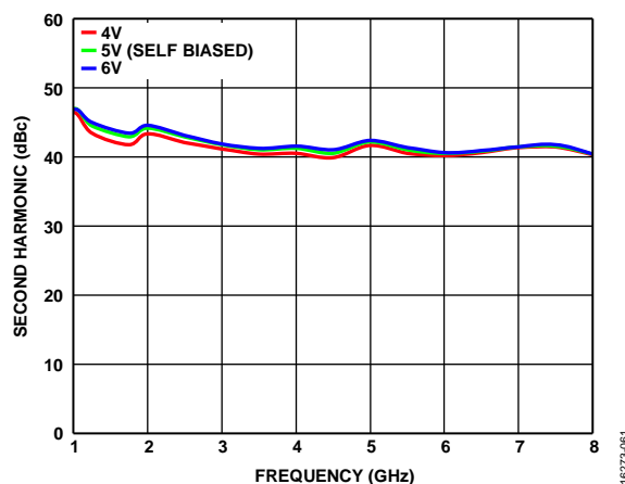
Figure 61. Second Harmonic vs. Frequency for Various V_{GG2} Values, V_{DD} = 12 V, V_{GG1} = \text{GND} , P_{OUT} = 10 dBm
