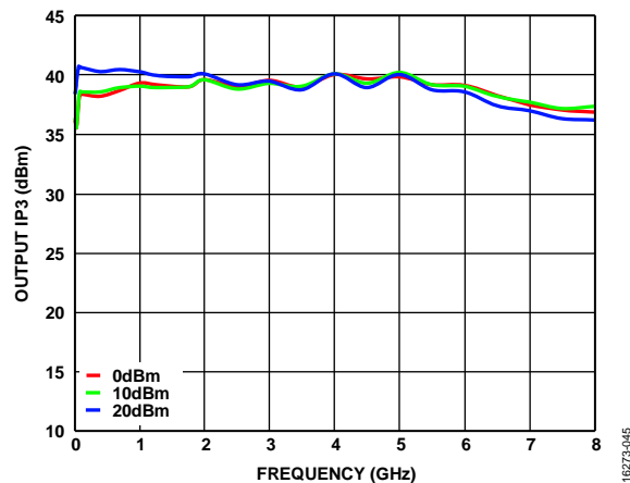
Figure 45. Output IP3 vs. Frequency for Various P_{OUT}/Tone , V_{DD} = 12\text{ V} , V_{GG2} = \text{Open} , V_{GG1} = \text{GND}
