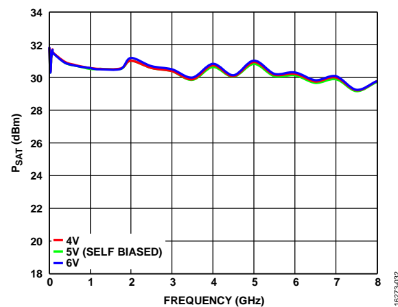
Figure 32. P_{SAT} vs. Frequency for Various V_{GG2} Values, V_{DD} = 12 V, V_{GG1} = \text{GND}
