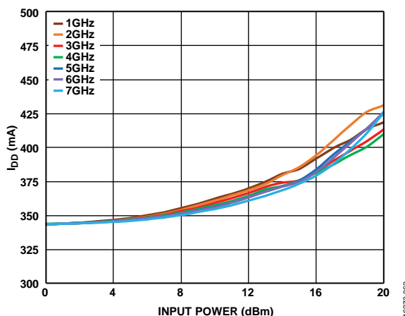
Figure 62. I_{DD} vs. Input Power for Various Frequencies, V_{DD} = 12 V, V_{GG2} = \text{Open} , V_{GG1} = \text{GND}
