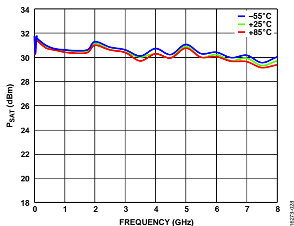
Figure 28. P_{SAT} vs. Frequency for Various Temperatures, Self Biased Mode, V_{DD} = 12 V, V_{GG2} = \text{Open} , V_{GG1} = \text{GND}
