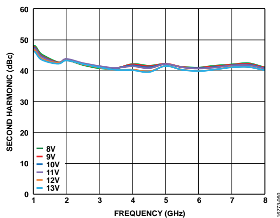
Figure 60. Second Harmonic vs. Frequency for Various Supply Voltages ( V_{DD} ), P_{OUT} = 10 dBm, V_{GG2} = \text{Open} , V_{GG1} = \text{GND}
