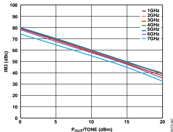
Figure 47. IM3 vs. P_{OUT}/Tone , V_{DD} = 11\text{ V} , V_{GG2} = \text{Open} , V_{GG1} = \text{GND}
