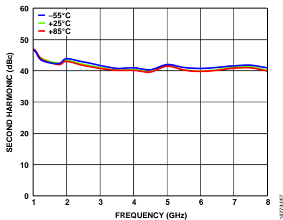
Figure 57. Second Harmonic vs. Frequency for Various Temperatures, P_{OUT} = 10 dBm, V_{DD} = 12 V, V_{GG2} = \text{Open} , V_{GG1} = \text{GND} (Self Biased)
