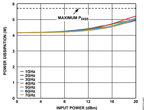
Figure 42. Power Dissipation vs. Input Power at T_A = 85^\circ\text{C} , V_{DD} = 12 V, V_{GG1} = GND , V_{GG2} = Open
