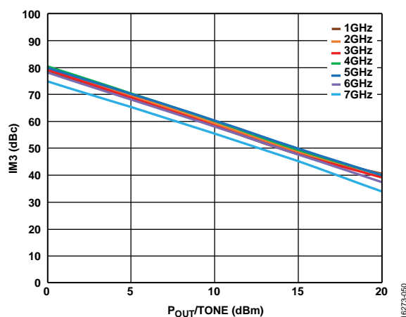
Figure 50. IM3 vs. P_{OUT}/Tone , V_{DD} = 12\text{ V} , V_{GG2} = \text{Open} , V_{GG1} = \text{GND}
