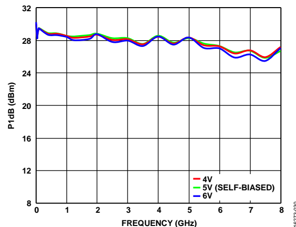
Figure 30. P1dB vs. Frequency for Various V_{GG2} Values, V_{DD} = 12 V, V_{GG1} = \text{GND}
