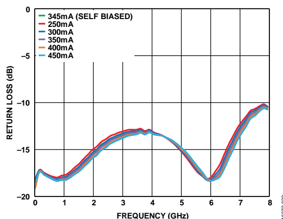
Figure 20. Output Return Loss vs. Frequency for Various Supply Currents ( I_{DD} ), External Biased condition, V_{DD} = 12 V, V_{GG2} = Open, Controlled V_{GG1}
