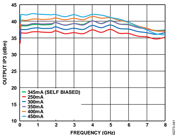
Figure 41. Output IP3 vs. Frequency for Various Supply Current ( I_{DD} ), V_{DD} = 12 V, V_{GG2} = Open , Controlled V_{GG1} , P_{OUT}/Tone = 10 dBm
