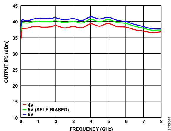
Figure 44. Output IP3 vs. Frequency for Various V_{GG2} Values, V_{DD} = 12 V, V_{GG1} = GND , P_{OUT}/Tone = 10 dBm
