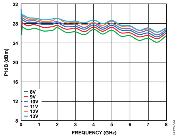
Figure 26. P1dB vs. Frequency for Various Supply Voltages ( V_{DD} ), V_{GG2} = \text{Open} , V_{GG1} = \text{GND}
