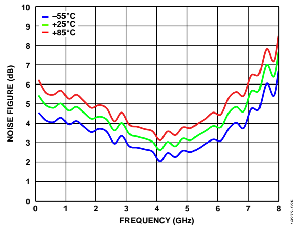
Figure 25. Noise Figure vs. Frequency for Various Temperatures, Self Biased Mode, V_{DD} = 12\text{ V} , V_{GG2} = \text{Open} , V_{GG1} = \text{GND}
