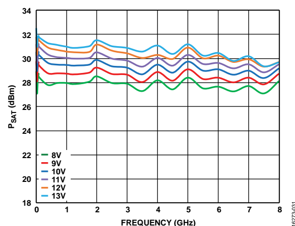
Figure 31. P_{SAT} vs. Frequency for Various Supply Voltages ( V_{DD} ), V_{GG2} = \text{Open} , V_{GG1} = \text{GND}
