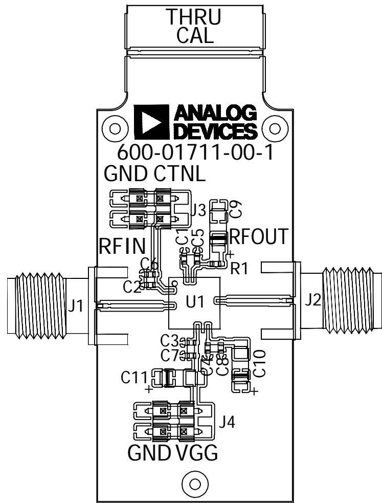
Figure 71. Evaluation PCB
