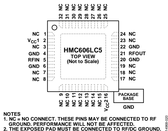
Figure 2. Pin Configuration
