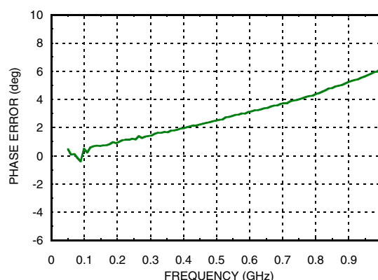
Phase Balance *
