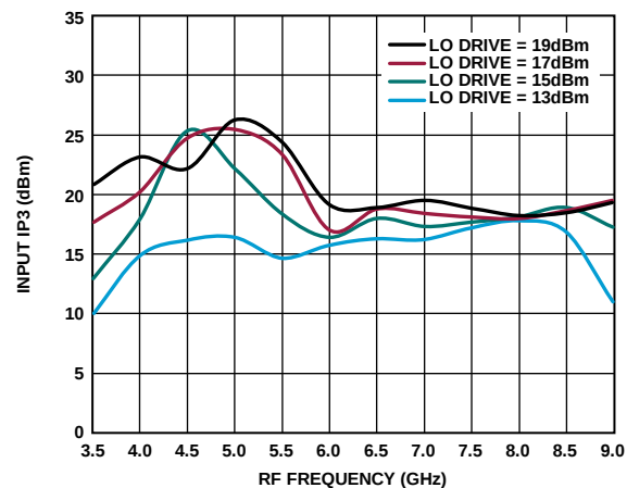
Figure 85. Input IP3 vs. RF Frequency at Various LO Drives, T_A = 25^\circ\text{C}
