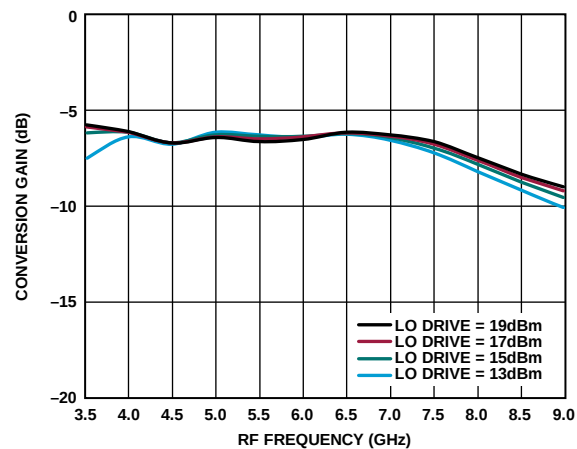
Figure 83. Conversion Gain vs. RF Frequency at Various LO Drives, T_A = 25^\circ\text{C}
