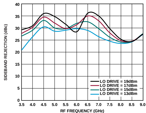
Figure 84. Sideband Rejection vs. RF Frequency at Various LO Drives, T_A = 25^\circ\text{C}
