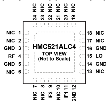
Figure 2. Pin Configuration
