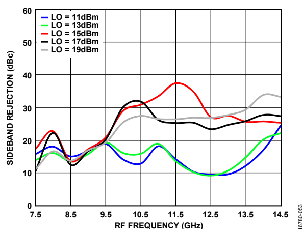
Figure 53. Sideband Rejection vs. RF Frequency at Various LO Power Levels, T A = 25°C
