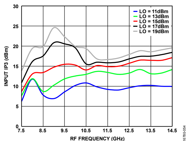
Figure 54. Input IP3 vs. RF Frequency at Various LO Power Levels, T A = 25°C
