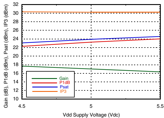
Gain, Power & Output IP3 vs. Supply Voltage @ 22 GHz
