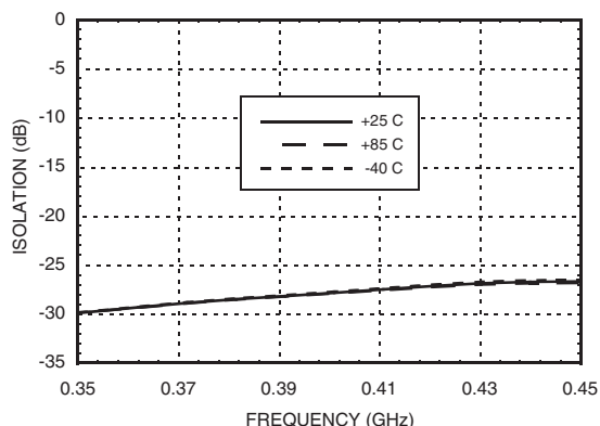
Reverse Isolation vs. Temperature @ 400 MHz
