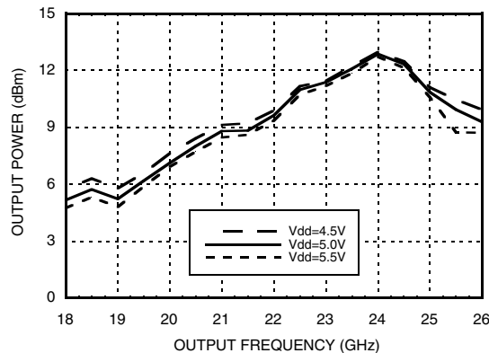
Output Power vs. Supply Voltage @ 0 dBm Drive Level
