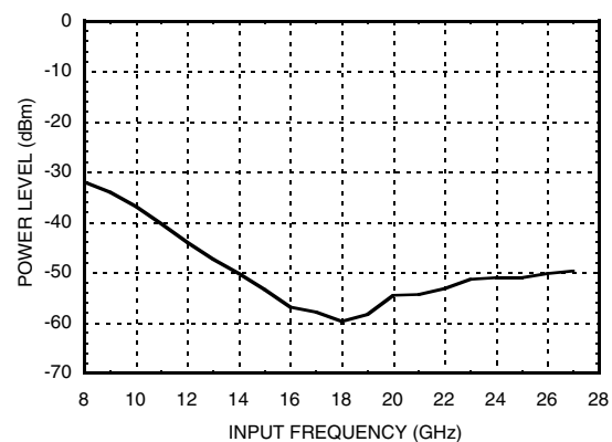
Reverse Leakage, P_{in} = 0\text{ dBm} , T = 25^\circ\text{C} Output Port Terminated
