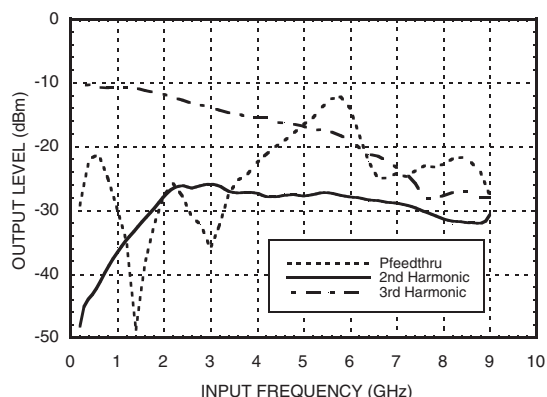
Output Harmonic
