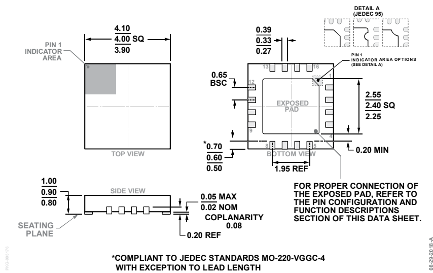
Figure 26. 16-Lead Lead Frame Chip Scale Package [LFCSP] 4 mm × 4 mm Body and 0.90 mm Package Height (CP-16-40)
