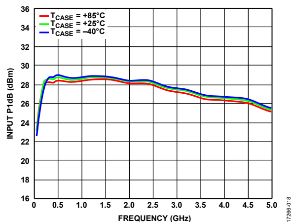
Figure 18. Input P1dB vs. Frequency over Temperature, V_{DD} = 3\text{ V}
