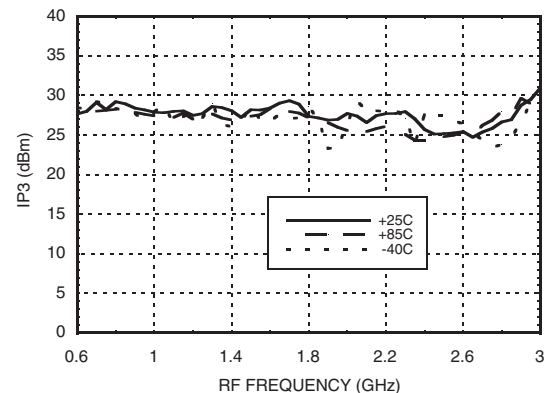
Input IP3 vs. Temperature @ LO = 0 dBm, IF = 184 MHz, USB [2]
