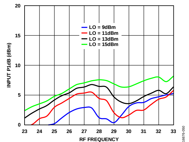
Figure 47. Input P1dB vs. RF Frequency at Various LO Power Levels, T_A = 25^\circ\text{C}
