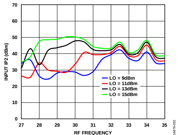
Figure 29. Input IP2 vs. RF Frequency at Various LO Power Levels, T_A = 25^\circ\text{C}
