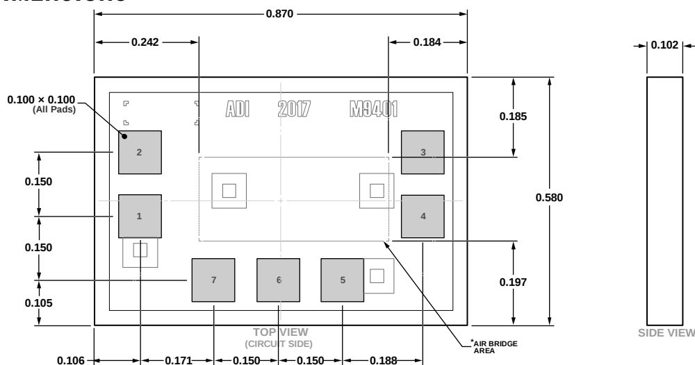
Figure 81. 7-Pad Bare Die [CHIP] (C-7-5)
