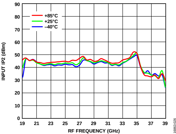
Figure 29. Input IP2 vs. RF Frequency at Various Temperatures, LO = 13 dBm
