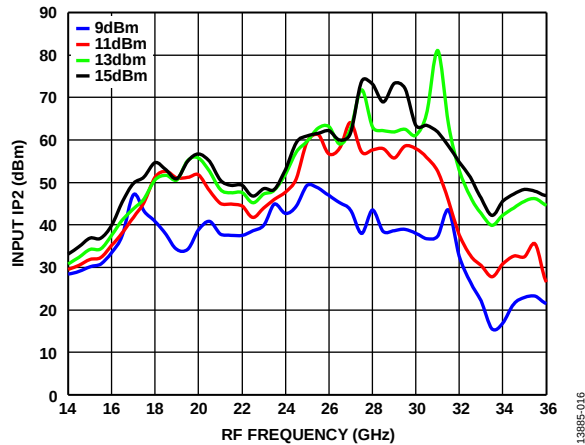
Figure 15. Input IP2 vs. RF Frequency at Various LO Power Levels, T_A = 25^\circ\text{C}
