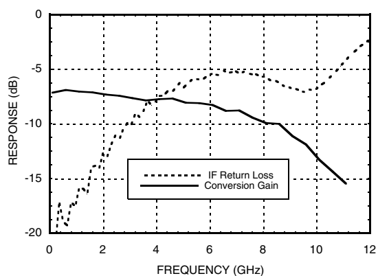
IF Bandwidth
