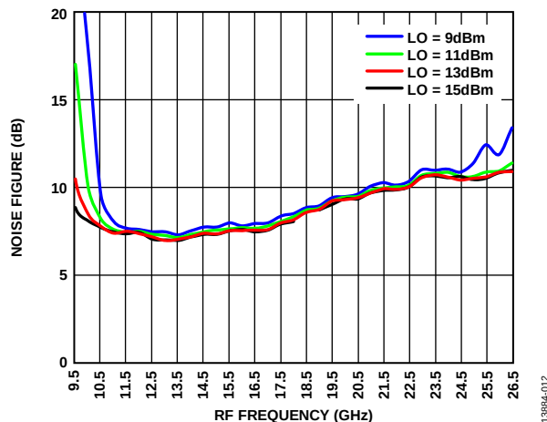
Figure 12. Noise Figure vs. RF Frequency at Various LO Power Levels, TA = 25°C
