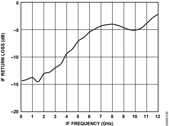
Figure 30. IF Return Loss vs. IF Frequency
