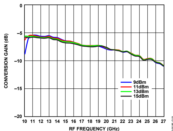
Figure 19. Conversion Gain vs. RF Frequency at Various LO Powers
