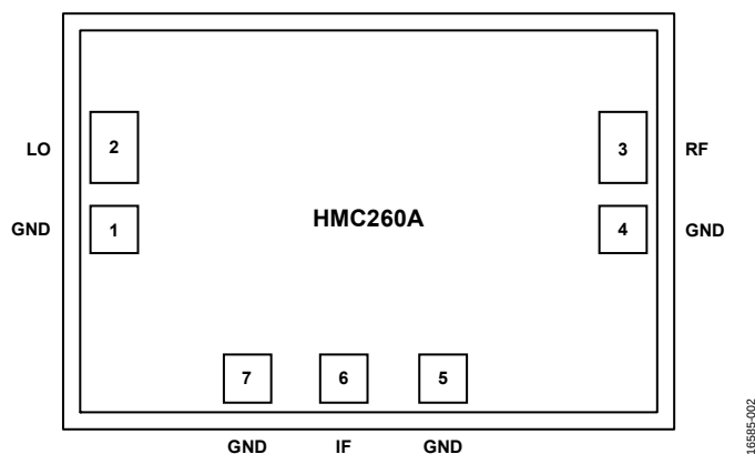
Figure 2. Pin Configuration
