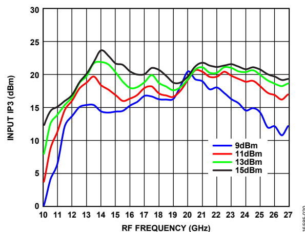
Figure 20. Input IP3 vs. RF Frequency at Various LO Powers
