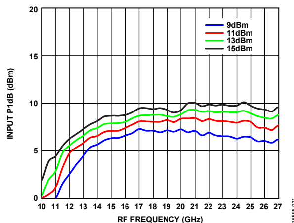
Figure 21. Input P1dB vs. RF Frequency at Various LO Powers
