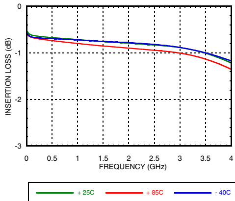
Insertion Loss
