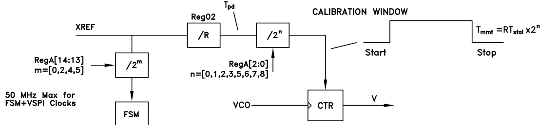
Figure 37. VCO Calibration
