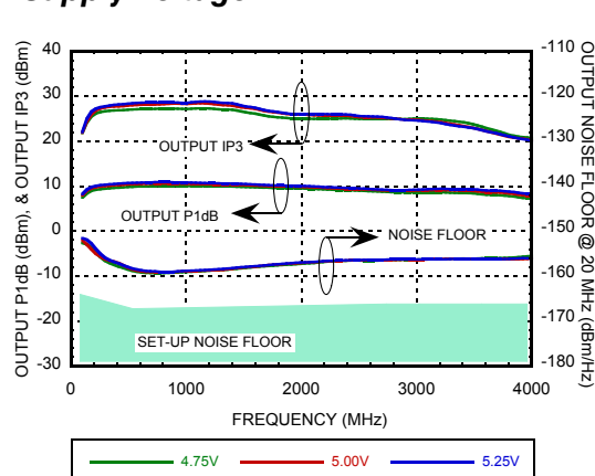
Figure 12. RF Output IP3, P1dB & NoiseFloor @ 20 MHz Offset vs. Frequency Over Supply Voltage
