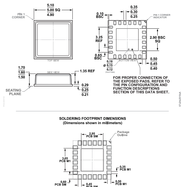
Figure 68. 24-Terminal Chip Array Small Outline No Lead Cavity [LGA_CAV] 5.00 mm x 5.00 mm Body and 1.60 mm Package Height (CE-24-2) Dimensions shown in millimeters
