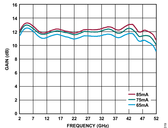
Figure 19. Gain vs. Frequency at Various I_{DQ} Currents, V_{DD} = 5 V, V_{GG2} = 1 V
