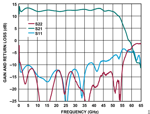
Figure 11. Gain and Return Loss vs. Frequency, V_{DD} = 5 V, I_{DQ} = 85 mA, V_{GG2} = 1 V
