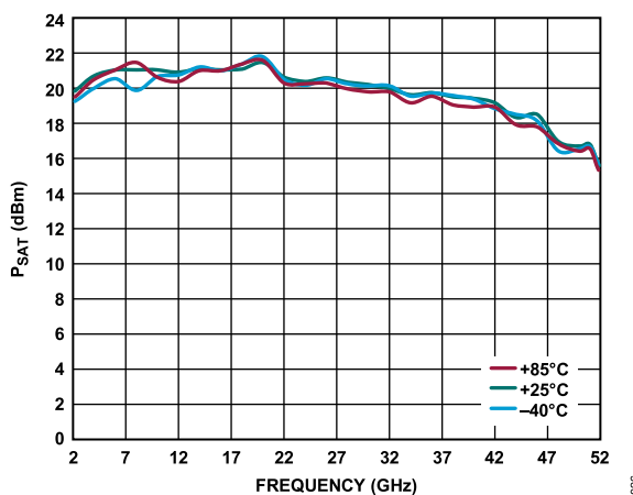
Figure 31. P_{SAT} vs. Frequency at Various Temperatures, V_{DD} = 5 V, I_{DQ} = 85 mA, V_{GG2} = 1 V
