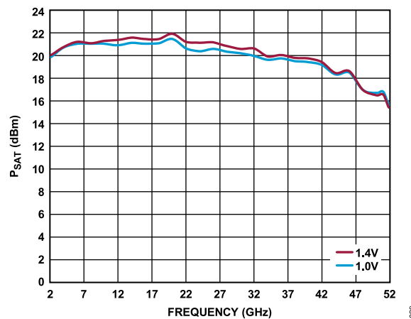
Figure 29. P_{SAT} vs. Frequency at Various V_{GG2} Voltages, V_{DD} = 5 V, I_{DQ} = 85 mA
