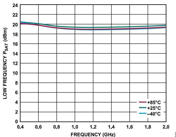
Figure 28. Low Frequency P_{SAT} vs. Frequency at Various Temperatures, V_{DD} = 5 V, I_{DQ} = 85 mA, V_{GG2} = 1 V
