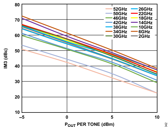
Figure 44. IM3 vs. P_{OUT} per Tone at Various Frequencies, V_{DD} = 5\text{ V} , I_{DQ} = 85\text{ mA} , V_{GG2} = 1\text{ V}
