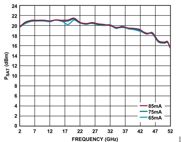
Figure 30. P_{SAT} vs. Frequency at Various I_{DQ} Currents, V_{DD} = 5 V, V_{GG2} = 1 V
