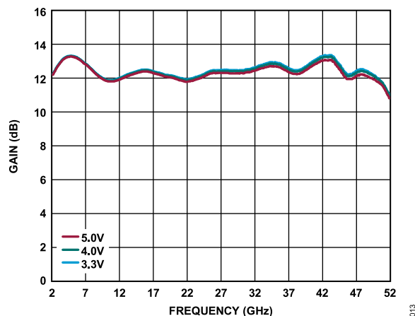
Figure 13. Gain vs. Frequency at Various V_{DD} Voltages, I_{DQ} = 85 mA, V_{GG2} = 1 V
