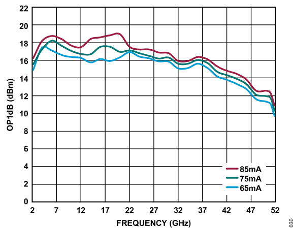
Figure 26. OP1dB vs. Frequency at Various I_{DQ} Currents, V_{DD} = 5 V, V_{GG2} = 1 V
