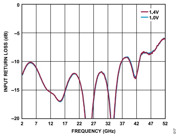
Figure 17. Input Return Loss vs. Frequency at Various V_{GG2} Voltages, V_{DD} = 5 V, I_{DQ} = 85 mA
