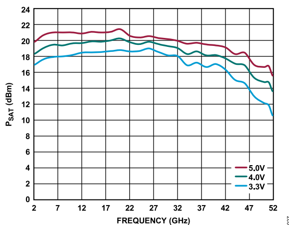
Figure 27. P_{SAT} vs. Frequency at Various V_{DD} Voltages, I_{DQ} = 85 mA, V_{GG2} = 1 V
