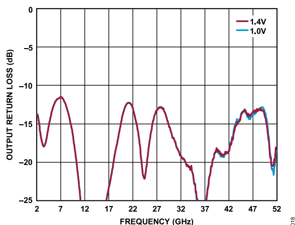
Figure 18. Output Return Loss vs. Frequency at Various V_{GG2} Voltages, V_{DD} = 5 V, I_{DQ} = 85 mA
