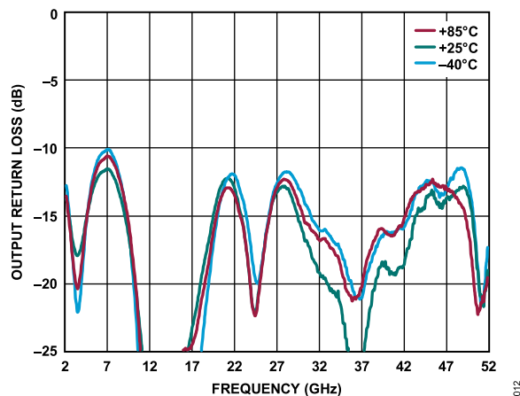
Figure 12. Output Return Loss vs. Frequency at Various Temperatures, V_{DD} = 5 V, I_{DQ} = 85 mA, V_{GG2} = 1 V
