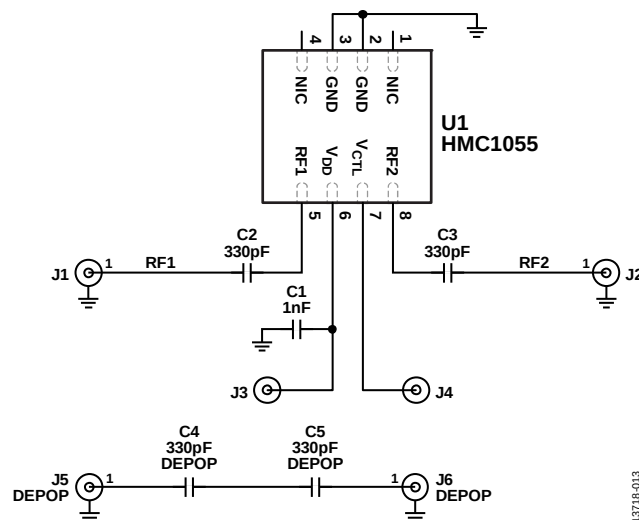
Figure 13. Evaluation Board Schematic
