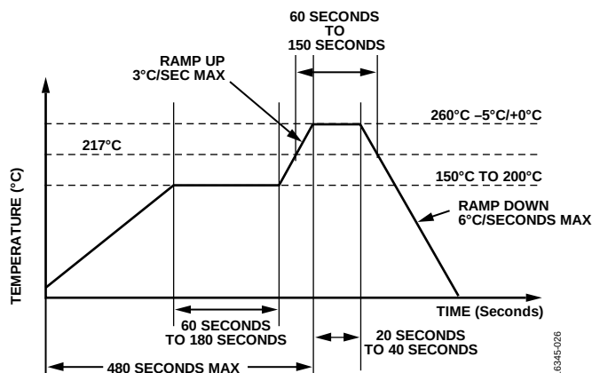
Figure 2. Pb-Free Reflow Solder Profile
