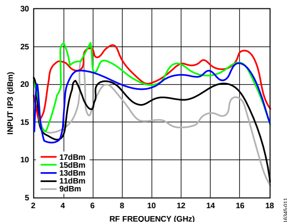
Figure 12. Input IP3 vs. RF Frequency over LO Drive at f_{IF} = 100 MHz, T_A = 25^\circ\text{C}
