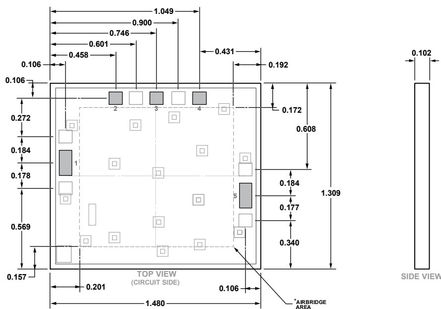
Figure 36. 5-Pad Bare Die [CHIP] (C-5-6)
