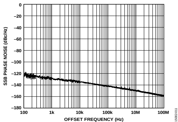
Figure 12. SSB Phase Noise vs. Offset Frequency, f_{OUT} = 15\text{ GHz} , Input Power = 6 dBm
