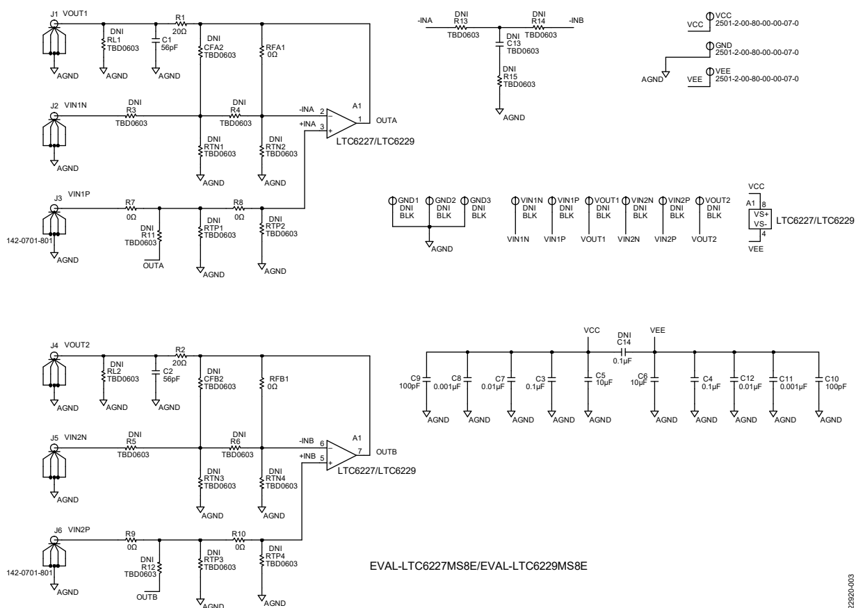
Figure 5. EVAL-LTC6227MS8E/EVAL-LTC6229MS8E Schematic
