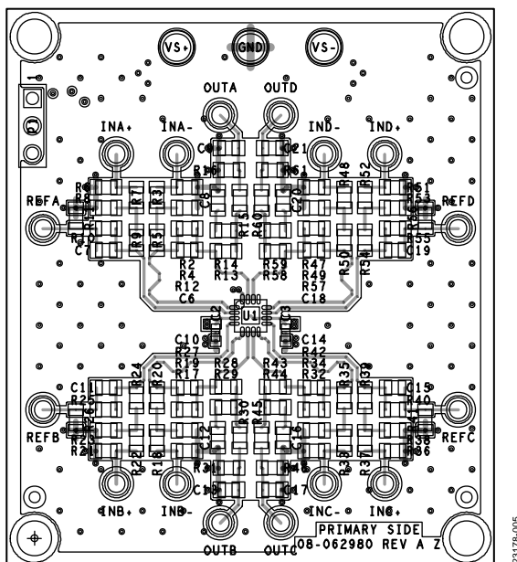
Figure 5. EVAL-LTC2065/LTC2068-TQFN Layout Pattern, Primary Side
