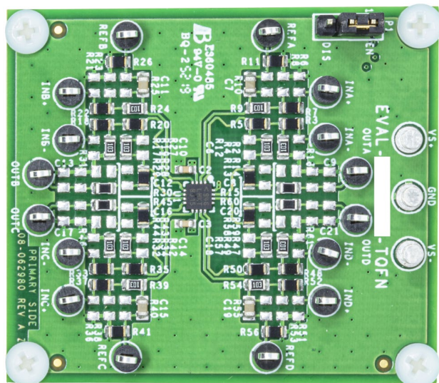
Figure 1. EVAL-LTC2065/LTC2068-TQFN, Primary Side
