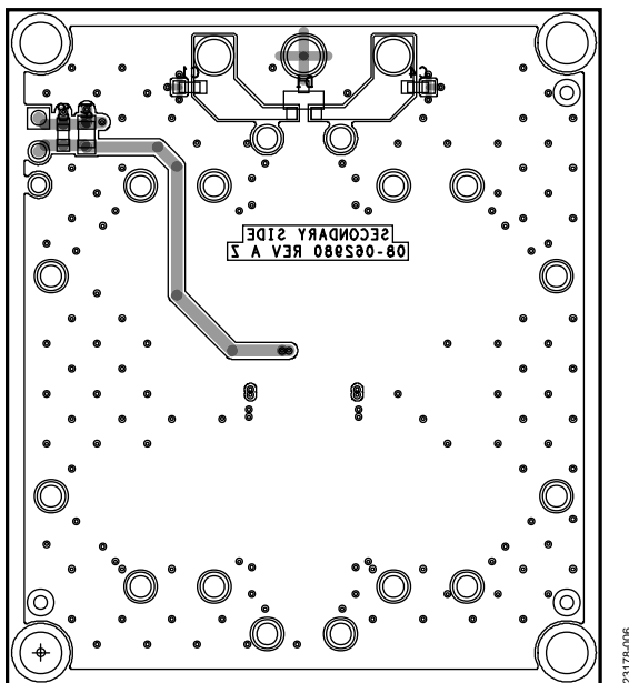
Figure 6. EVAL-LTC2065/LTC2068-TQFN Layout Pattern, Secondary Side
