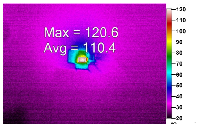
Figure 14. Thermal Image of Bottom Layer at 24V OUT , 10A I OUT , 1MHz (Forced Airflow, Thermal Values are on Q1)
