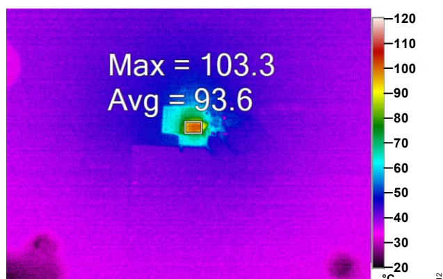
Figure 12. Thermal Image of Bottom Layer at 24V OUT , 5A I OUT , 1MHz. (Thermal Values are on Q1)
