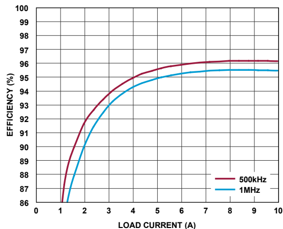
Figure 4. Efficiency vs. Load Current at 12V OUT (Forced Airflow)
