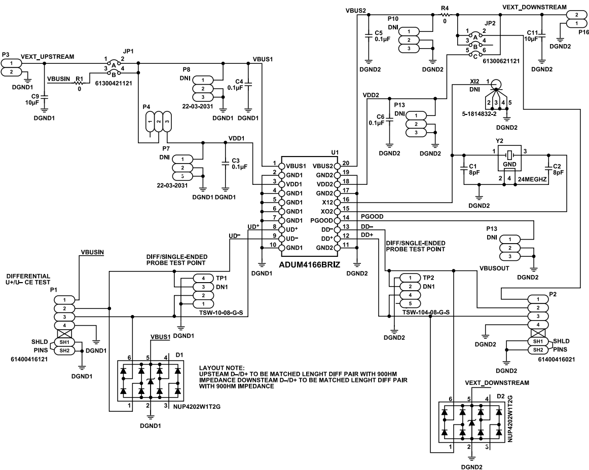
Figure 6. EVAL-ADuM4166EBZ Schematic
